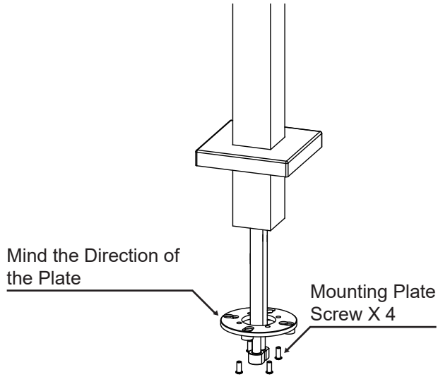
Installation of Floor Mounting Plate
